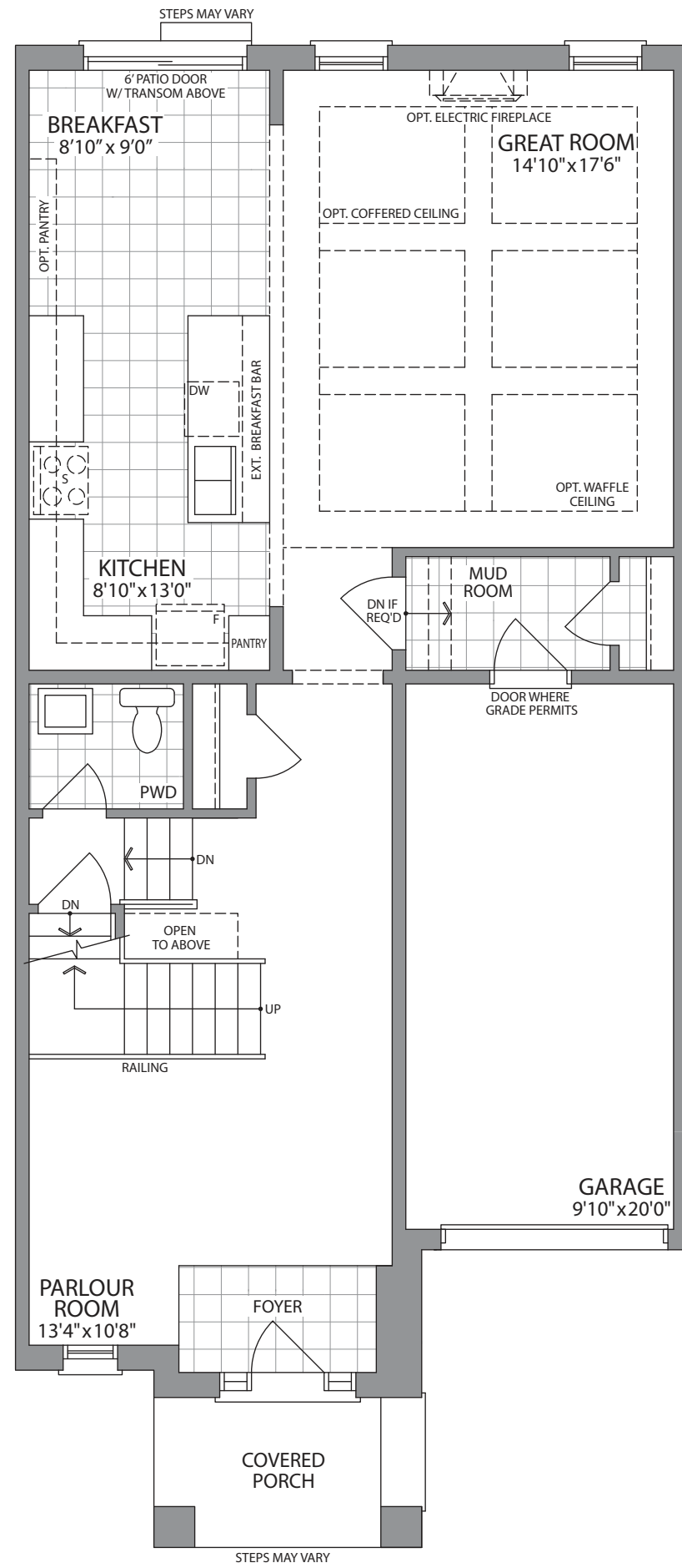
GROUND FLOOR PLAN STYLE 'C'
