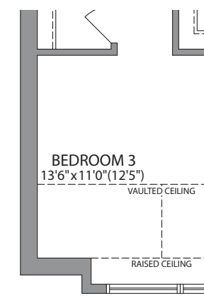
SECOND FLOOR PLAN STYLE 'E' END
