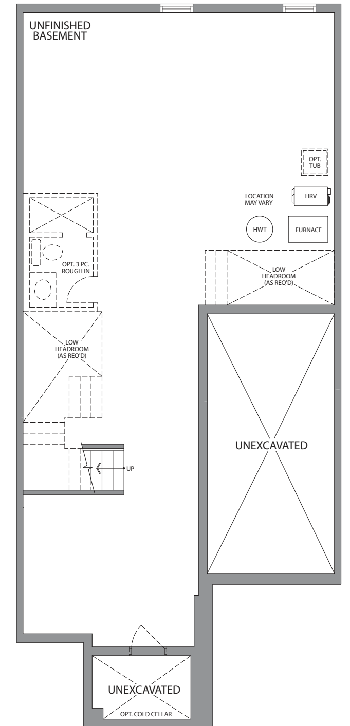
BASEMENT STYLE 'C'
