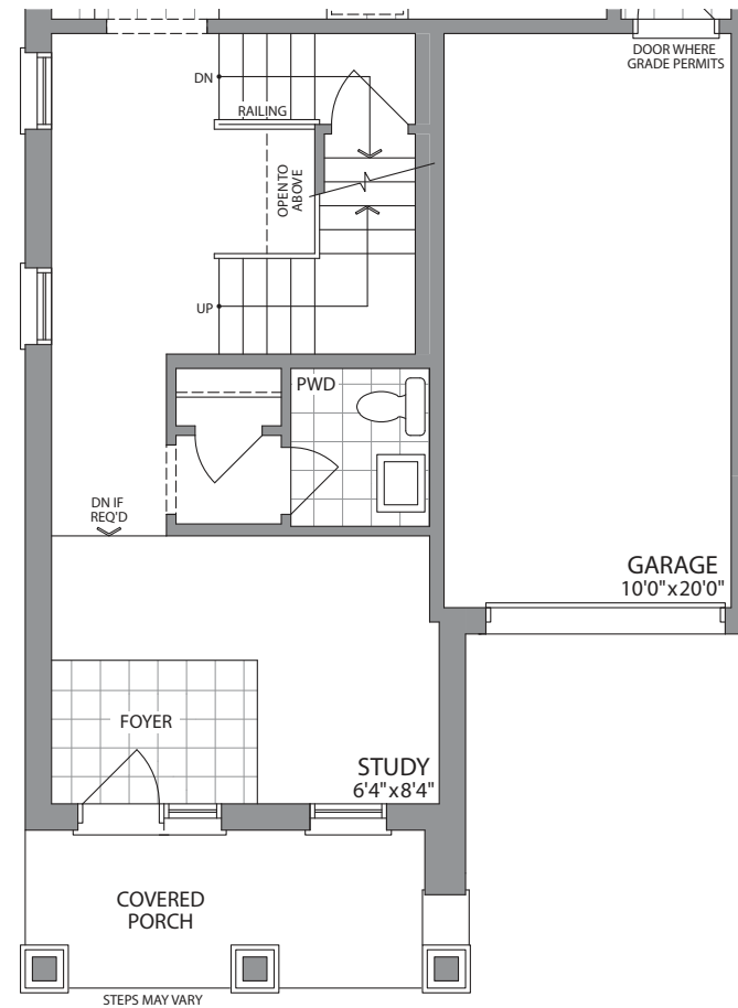
GROUND FLOOR PLAN STYLE 'E' END
