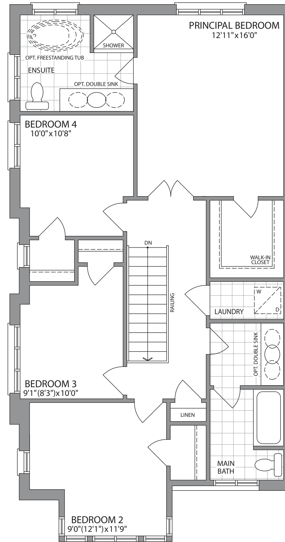
SECOND FLOOR PLAN STYLE 'C'
