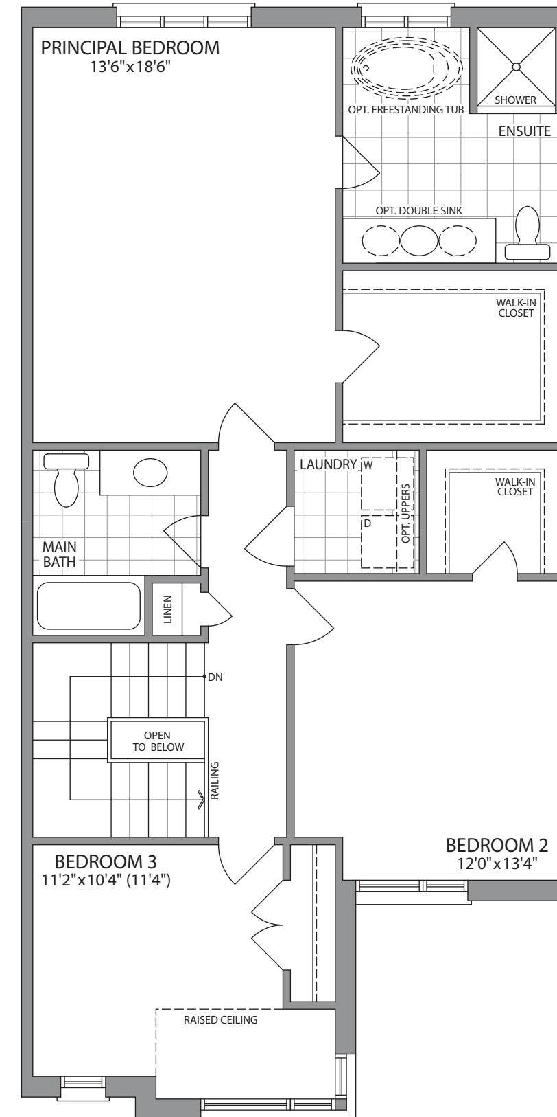
SECOND FLOOR PLAN STYLE 'C'
