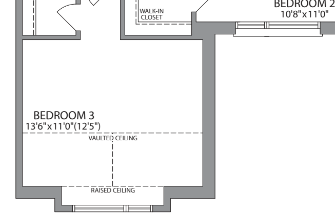
SECOND FLOOR PLAN STYLE 'E' INTERIOR
