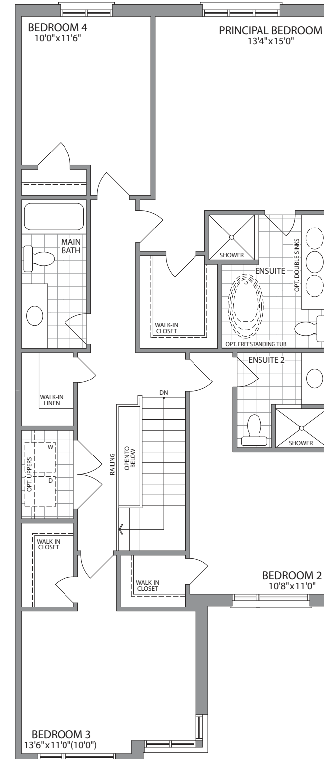
SECOND FLOOR PLAN STYLE 'C' INTERIOR
