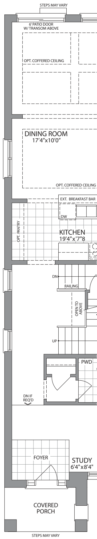
GROUND FLOOR PLAN STYLE 'C' END
