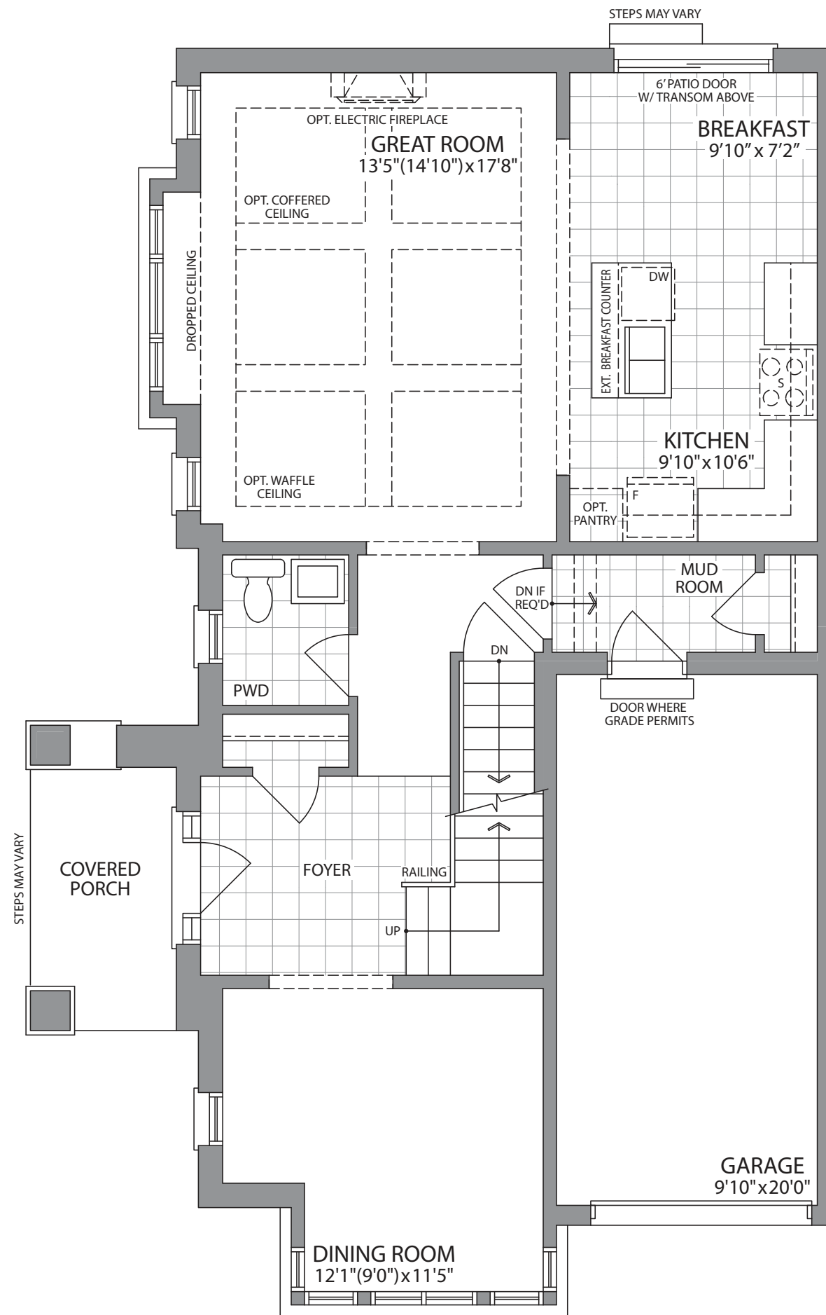
GROUND FLOOR PLAN STYLE 'C'
