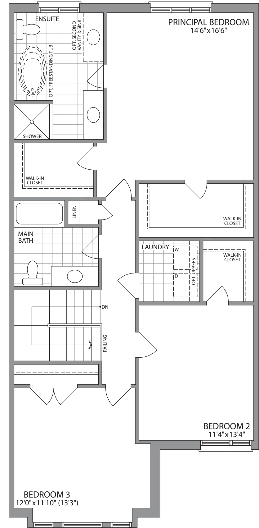
SECOND FLOOR PLAN STYLE 'C'
