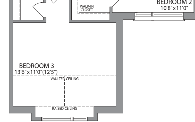
SECOND FLOOR PLAN STYLE 'E' INTERIOR
