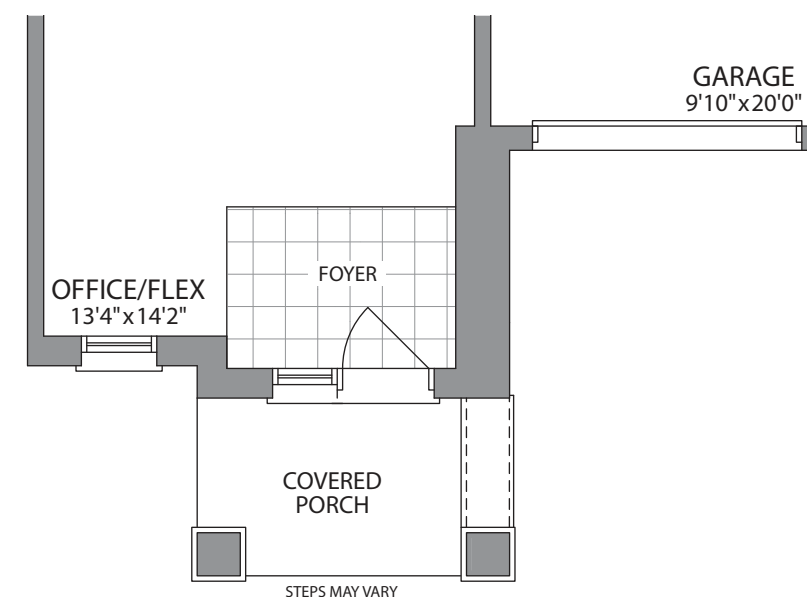
GROUND FLOOR PLAN STYLE 'E'
