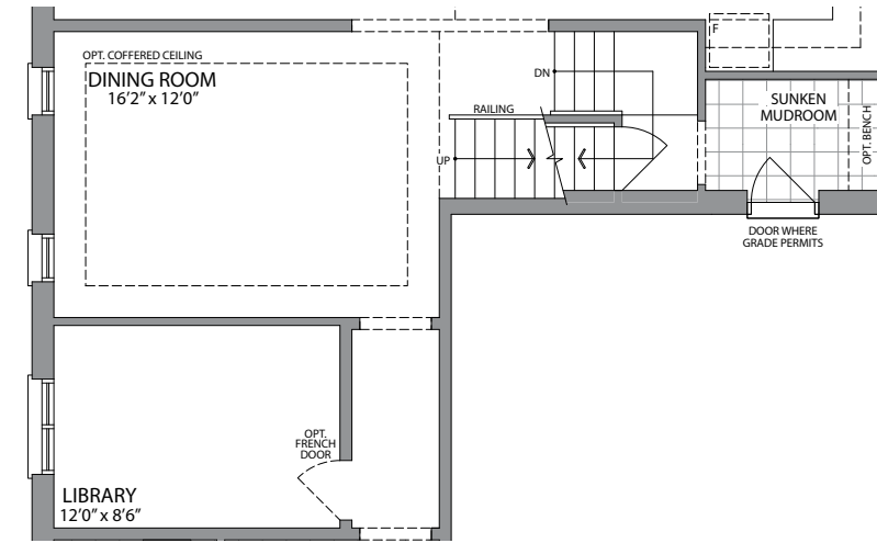
OPT. DINING & LIBRARY PLAN STYLE 'B', 'C', 'E' & 'A'
