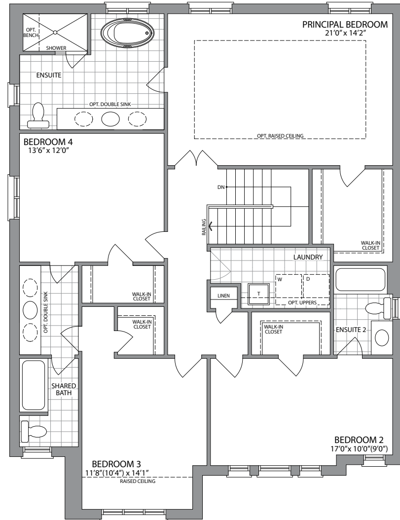
SECOND FLOOR PLAN (4 BED) STYLE 'B'
