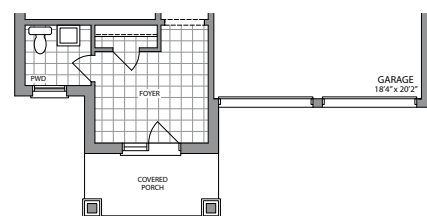
GROUND FLOOR PLAN STYLE 'E'
