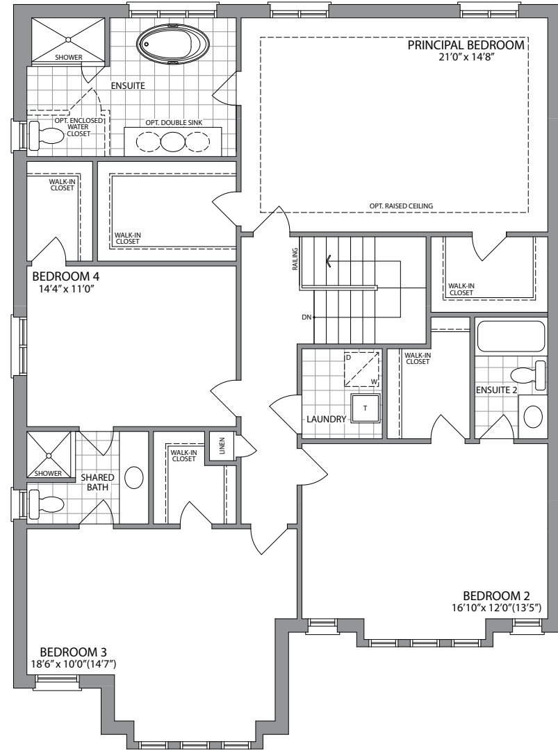
SECOND FLOOR PLAN (4 BED) STYLE 'B'
