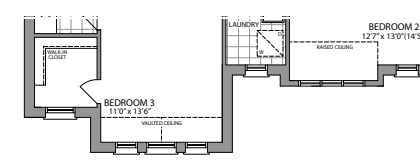
OPT. SECOND FLOOR PLAN STYLE 'D'
