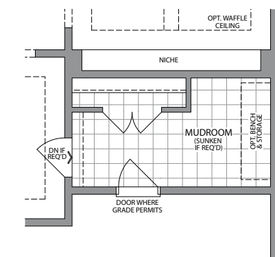
OPT. GROUND FLOOR PLAN FOR OPT. SECOND FLOOR PLAN STYLE 'E' (STYLE 'B', 'C' & 'D' SIMILAR)
