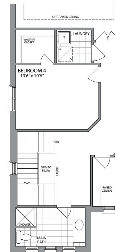
OPT. SECOND FLOOR PLAN W/OPT. MAIN BATH & LAUNDRY STYLE 'E' (STYLE 'B', 'C' & 'D' SIMILAR)
