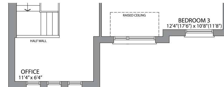
SECOND FLOOR PLAN STYLE 'E'
