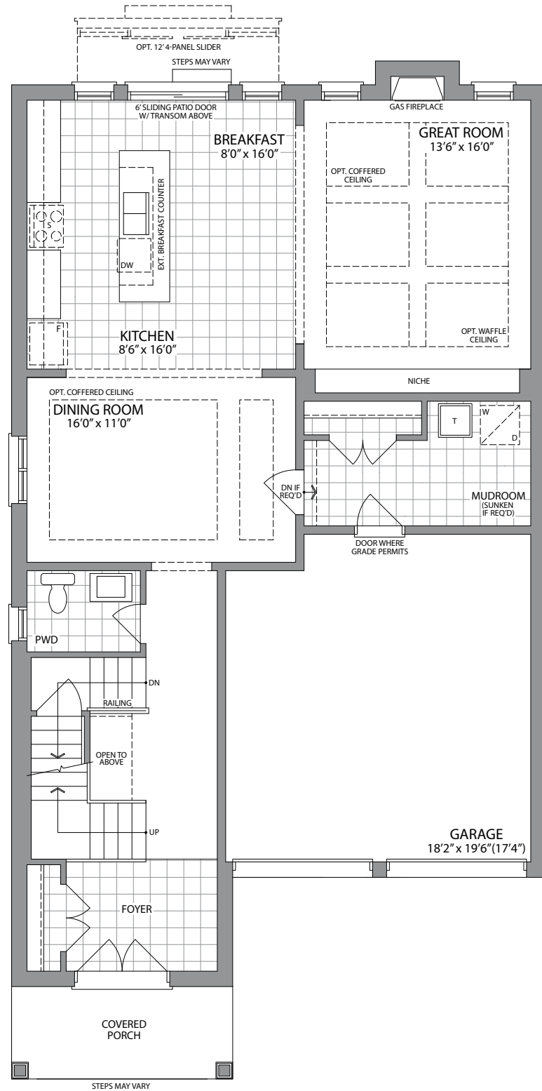
GROUND FLOOR PLAN STYLE 'B'
