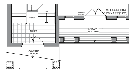
GROUND FLOOR PLAN STYLE 'D'
