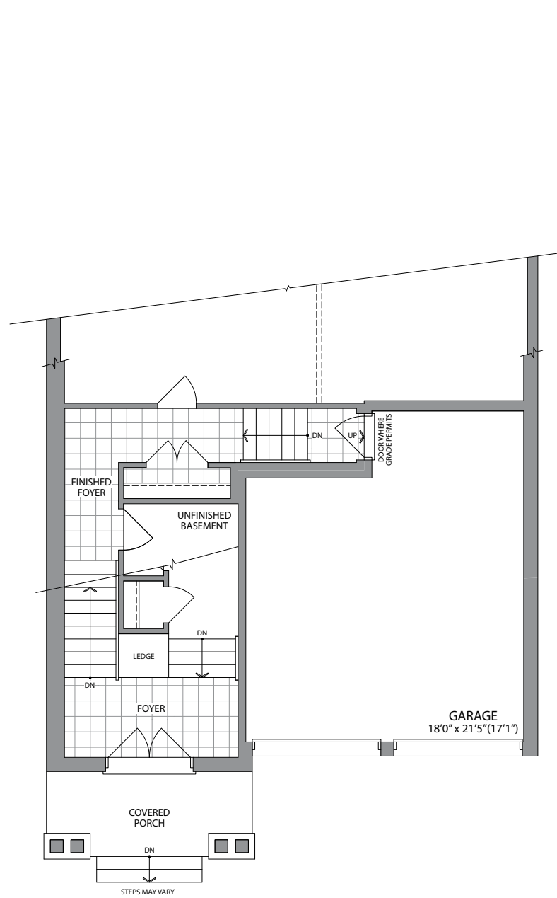
GARAGE LEVEL STYLE 'B' & 'E'
