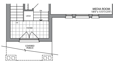
GROUND FLOOR PLAN STYLE 'E'
