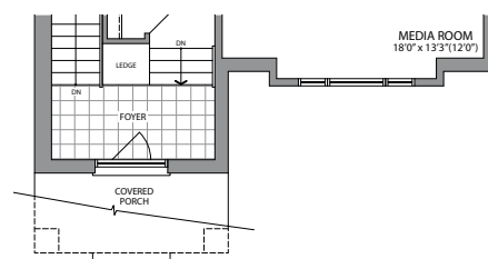
GROUND FLOOR PLAN STYLE 'C'
