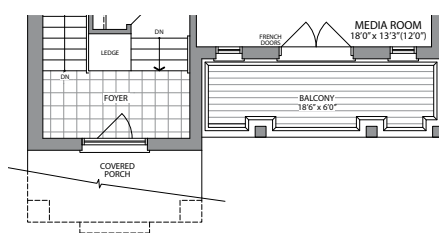
GROUND FLOOR PLAN STYLE 'C2'
