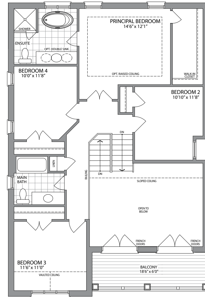
SECOND FLOOR PLAN STYLE 'B'
