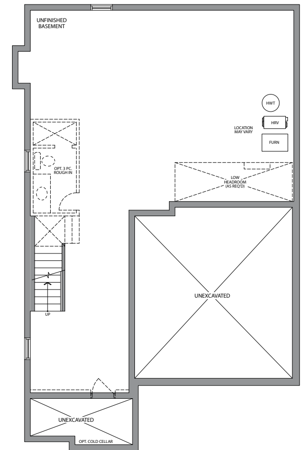
BASEMENT STYLE 'B' & 'E'
