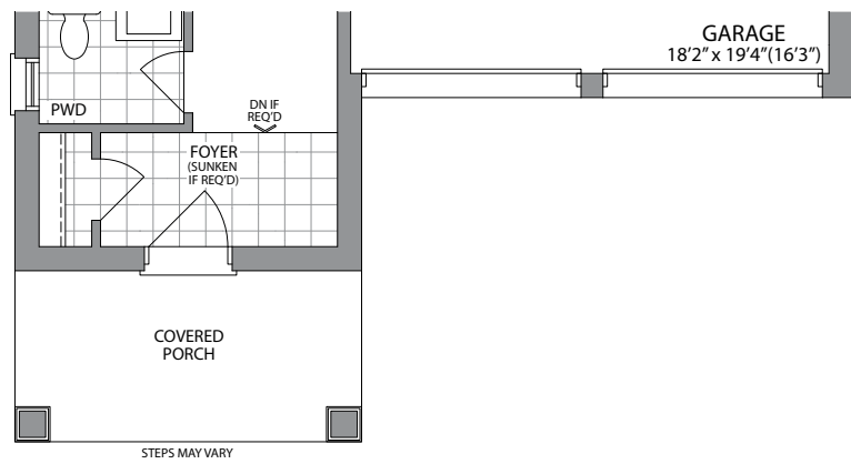
GROUND FLOOR PLAN STYLE 'D'
