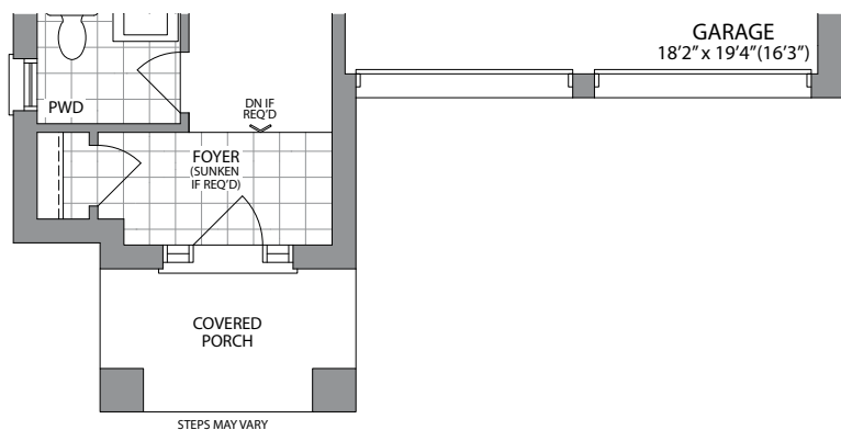
GROUND FLOOR PLAN STYLE 'C'
