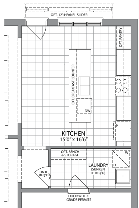
GROUND FLOOR PLAN W/OPT. CHEF'S KITCHEN
