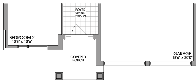
GROUND FLOOR PLAN ELEVATION 'C'
