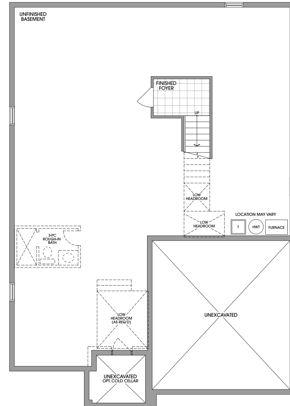
BASEMENT ELEVATION 'A' (ELEVATION 'C' & 'E' SIMILAR)
