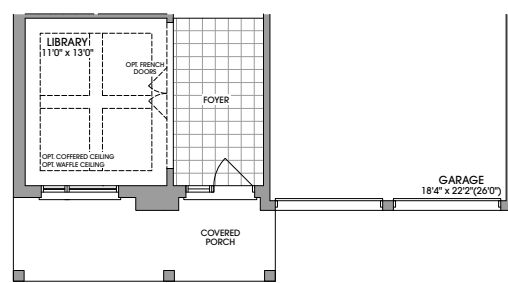
GROUND FLOOR PLAN ELEVATION 'B'
