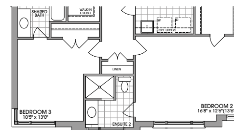
SECOND FLOOR PLAN ELEVATION 'C'
