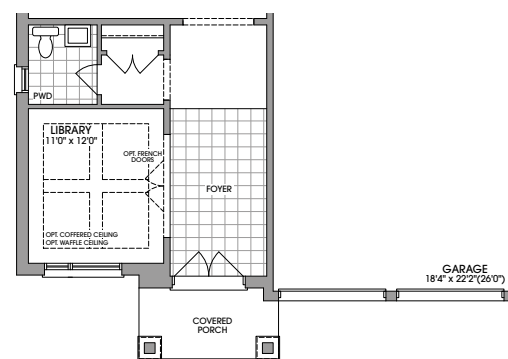
GROUND FLOOR PLAN ELEVATION 'C'
