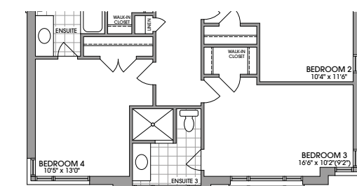
OPT. 5 BEDROOM PLAN ELEVATION 'C'
