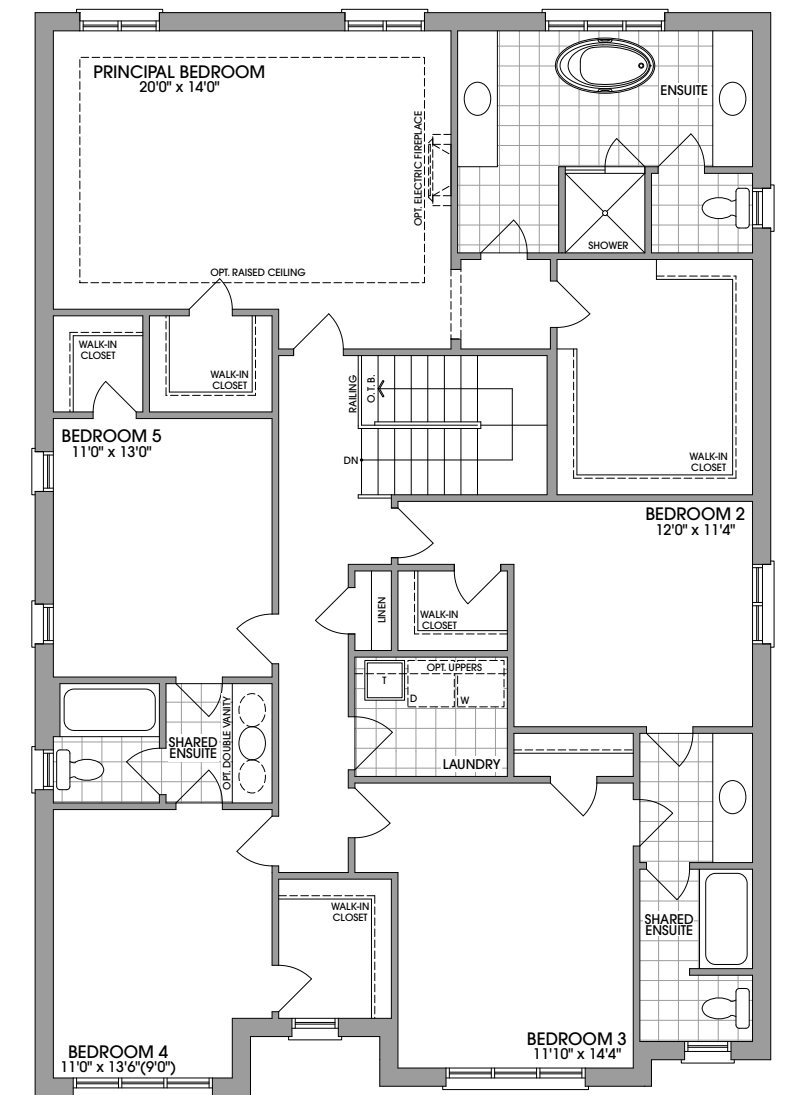
OPT. 5 BEDROOM PLAN ELEVATION 'A'
