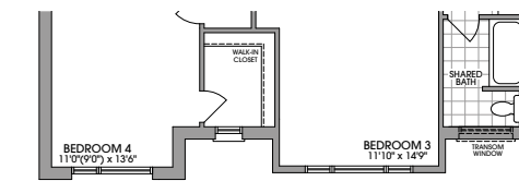
OPT. 5 BEDROOM PLAN ELEVATION 'C'
