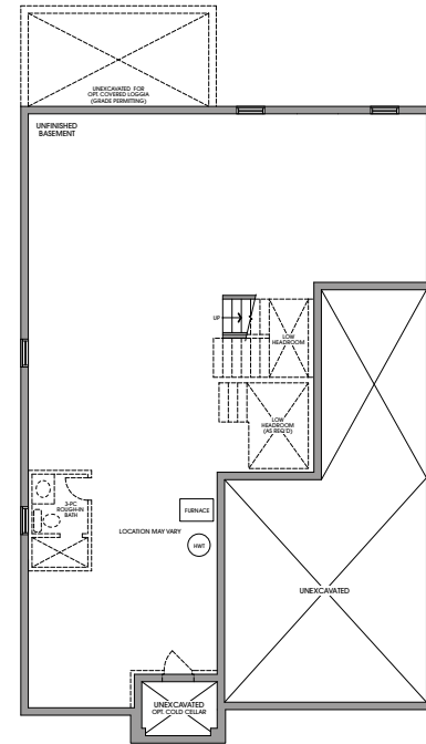
BASEMENT ELEVATION 'A' (ELEVATION 'B' & 'C' SIMILAR)
