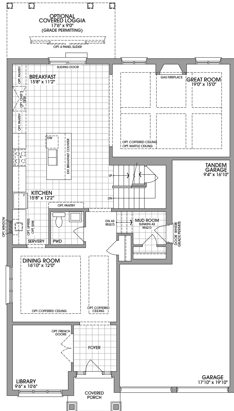
GROUND FLOOR PLAN ELEVATION 'A' (ELEVATION 'B' & 'C' SIMILAR)
