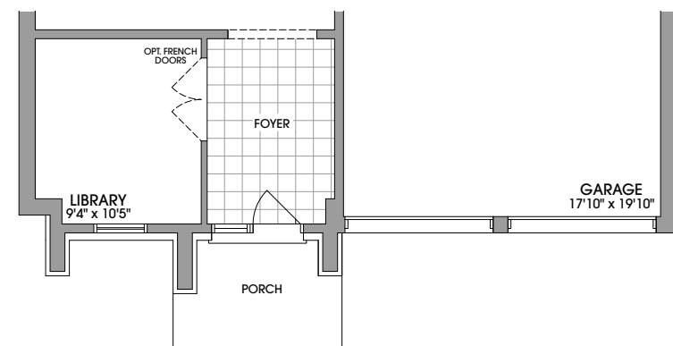
GROUND FLOOR PLAN ELEVATION 'E'
