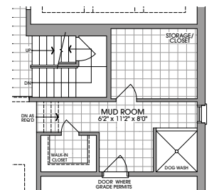
OPT. GROUND FLOOR PLAN W/DOG WASH ELEVATION 'A' (ELEVATION 'B, C & E' SIMILAR)
