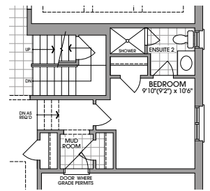
OPT. GROUND FLOOR PLAN W/BEDROOM ELEVATION 'A' (ELEVATION 'B, C & E' SIMILAR)
