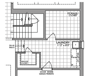
OPT. GROUND FLOOR PLAN W/ALT. MUDROOM & LAUNDRY LOCATION ELEVATION 'A' (ELEVATION 'B, C & E' SIMILAR)
