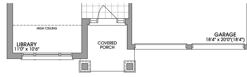
GROUND FLOOR PLAN ELEVATION 'C'
