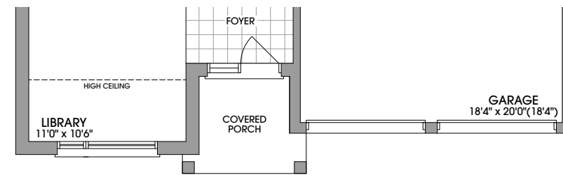
GROUND FLOOR PLAN ELEVATION 'B'
