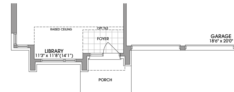
GROUND FLOOR PLAN ELEVATION 'E'
