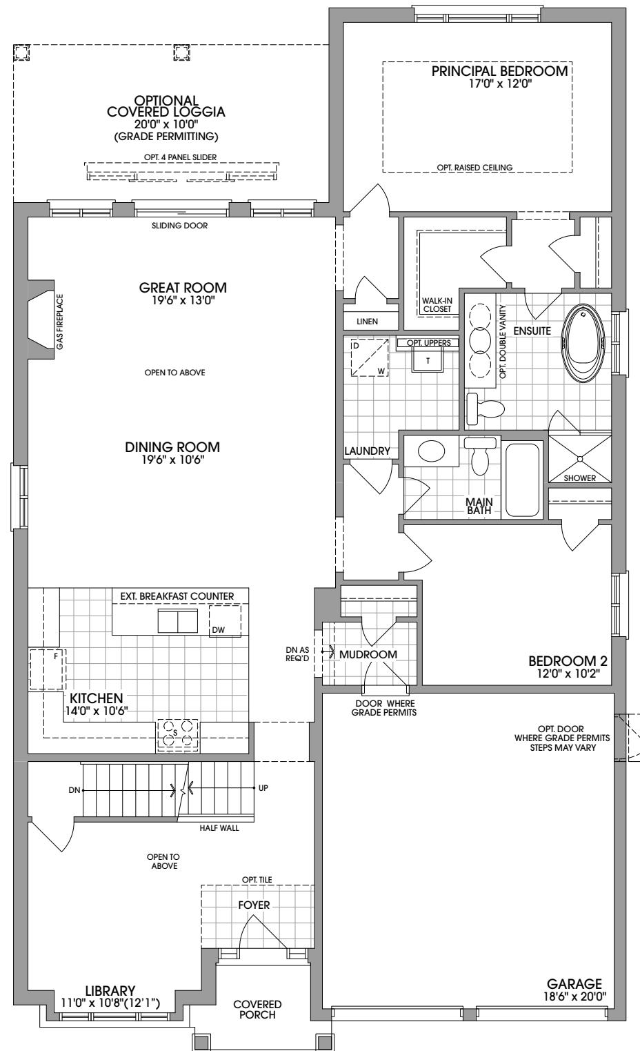
GROUND FLOOR PLAN ELEVATION 'A'
