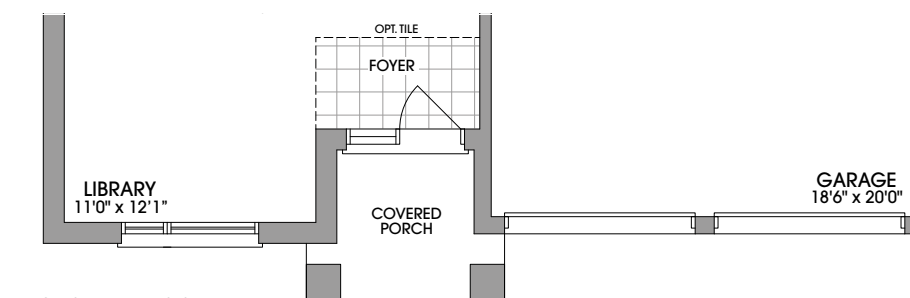
GROUND FLOOR PLAN ELEVATION 'B'
