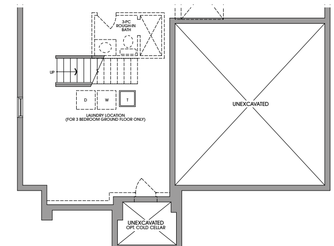
BASEMENT ELEVATION 'E'
