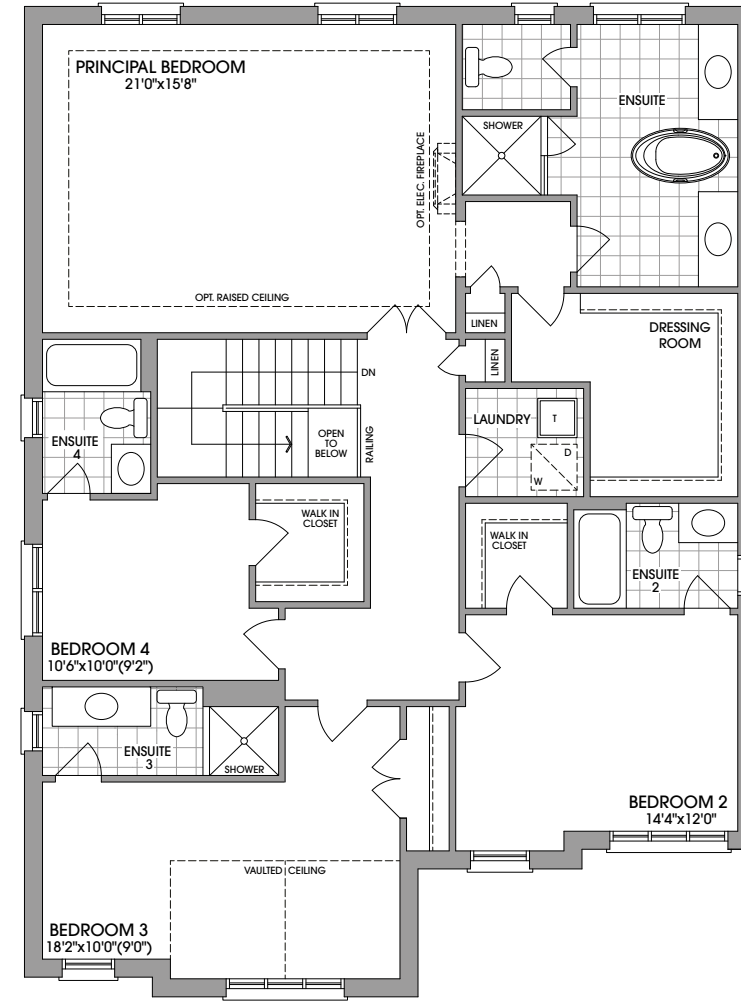
OPT. SECOND FLOOR W/ 4 BATHS FOR 4 BEDROOM PLAN ONLY ELEVATION 'B' (ELEVATION 'C' & 'E' SIMILAR)
