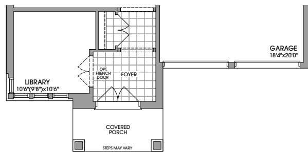
GROUND FLOOR PLAN ELEVATION 'C'
