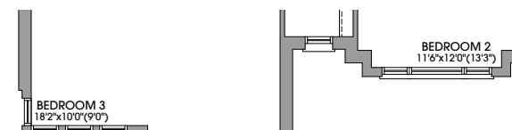
SECOND FLOOR PLAN ELEVATION 'C'
