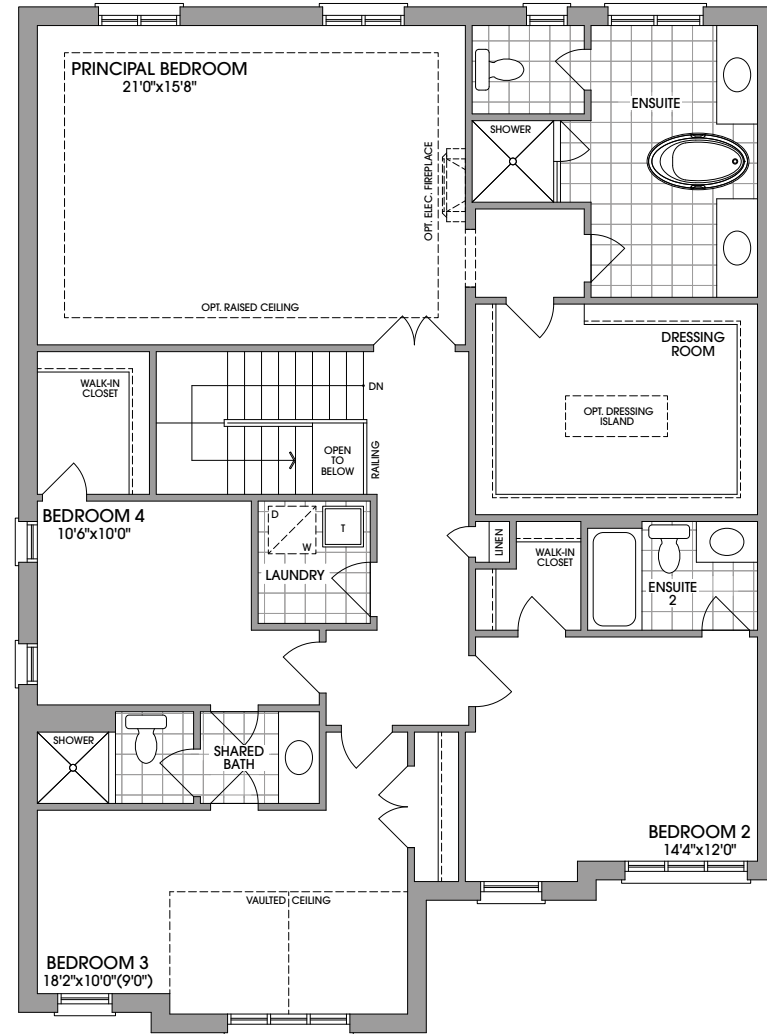
SECOND FLOOR PLAN ELEVATION 'B'
