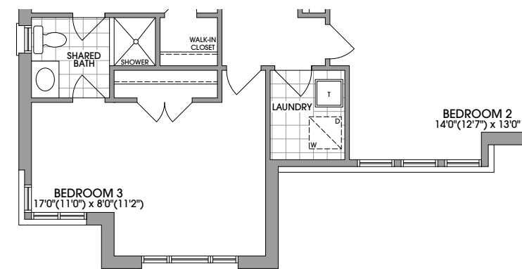
OPT. 5 BEDROOM PLAN ELEVATION 'C'
