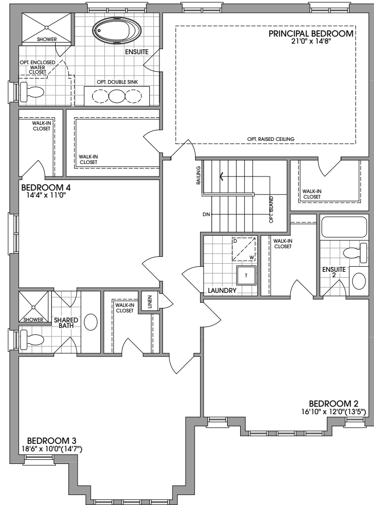
SECOND FLOOR PLAN ELEVATION 'B'
