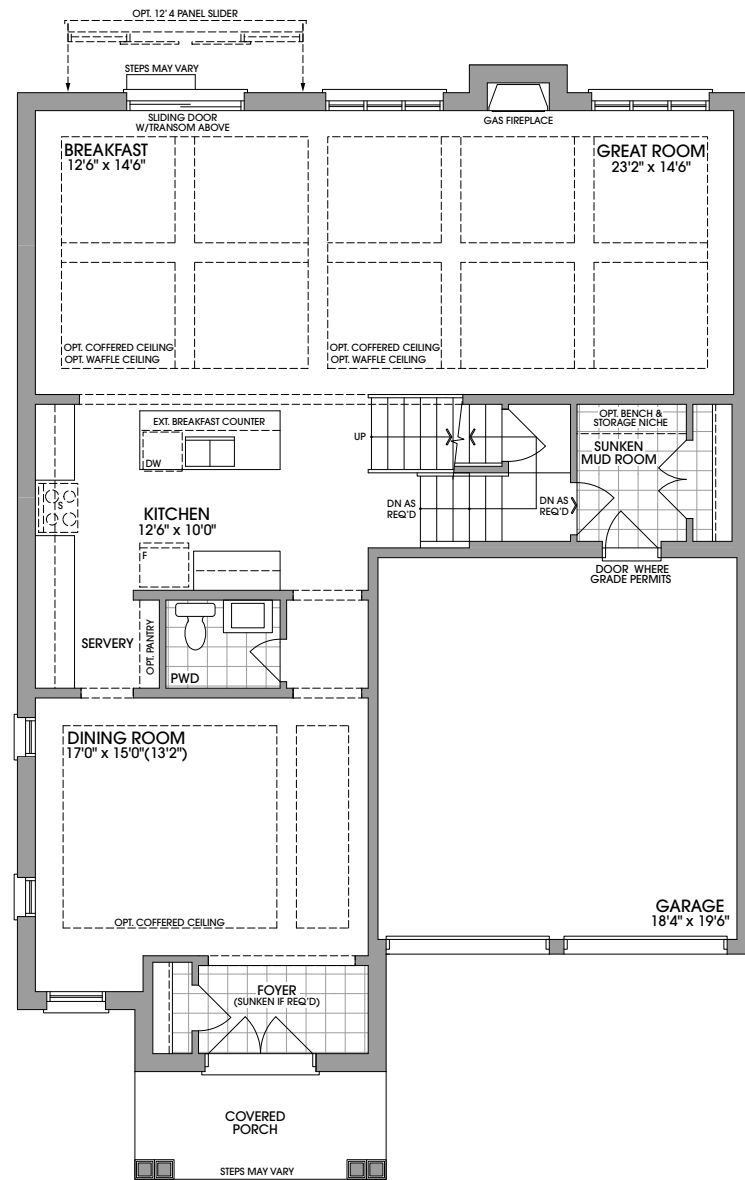
GROUND FLOOR PLAN ELEVATION 'B' (ELEVATION 'C' & 'E' SIMILAR)
