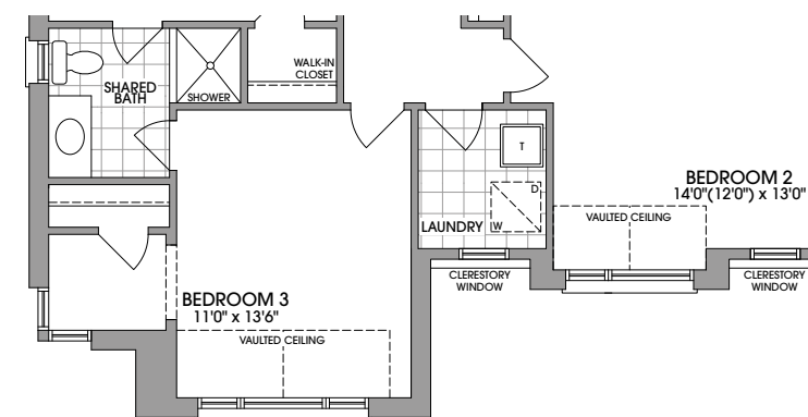
OPT. 5 BEDROOM PLAN ELEVATION 'E'
