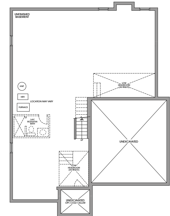
BASEMENT ELEVATION 'B' (ELEVATION 'C' & 'E' SIMILAR)
