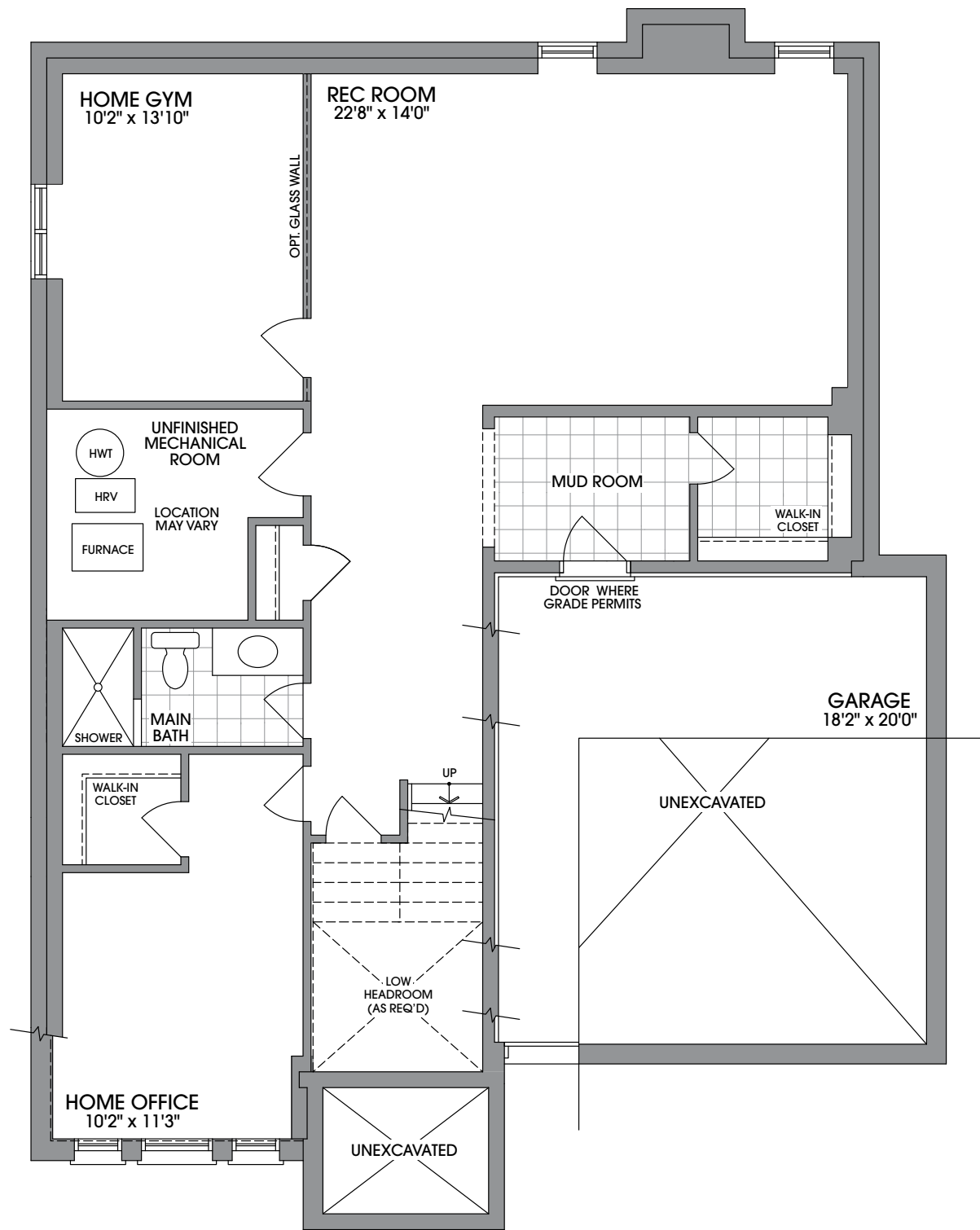
OPT. FINISHED BASEMENT ELEVATION 'B' (ELEVATION 'C' & 'E' SIMILAR)
