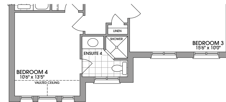
OPT. 5 BEDROOM PLAN W/ OPT. 4 BATH ELEVATION 'B' (ELEVATION 'C' & 'E' SIMILAR)
