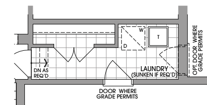
GROUND FLOOR PLAN W/ LAUNDRY ROOM RELOCATED FOR OPT. 4 BATH
