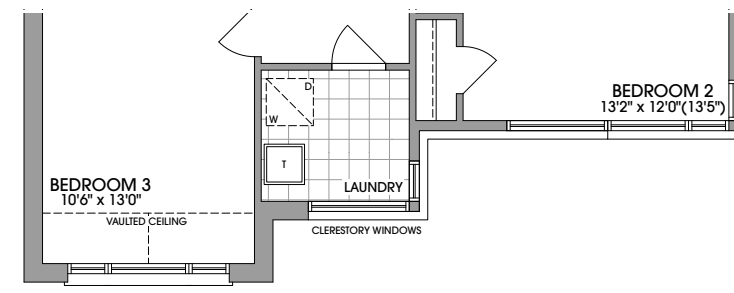
SECOND FLOOR PLAN ELEVATION 'E'
