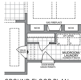
GROUND FLOOR PLAN FOR OPT. SECOND FLOOR STYLE 'B, C & D' SIMILAR
