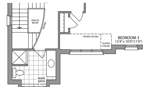
SECOND FLOOR PLAN STYLE 'D'
