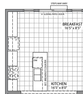
OPT. KITCHEN/ BREAKFAST LAYOUT STYLE 'B, C & D' SIMILAR
