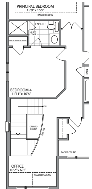
OPT. SECOND FLOOR W/OPT. ENSUITE AND OFFICE STYLE 'B, C & D' SIMILAR
