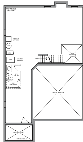
BASEMENT PLAN STYLE 'A' 'B & C' SIMILAR
