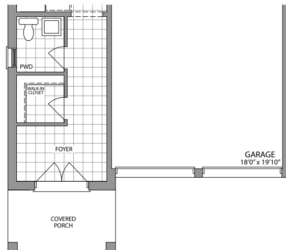
GROUND FLOOR PLAN STYLE 'C'
