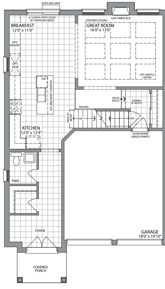
GROUND FLOOR PLAN STYLE 'B'
