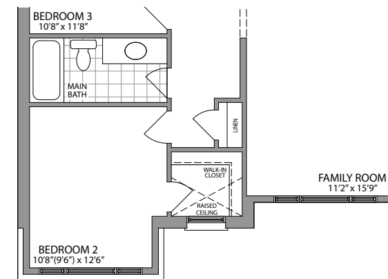
SECOND FLOOR PLAN STYLE 'C'
