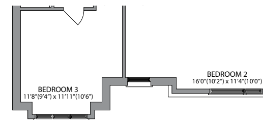
SECOND FLOOR PLAN STYLE 'C'
