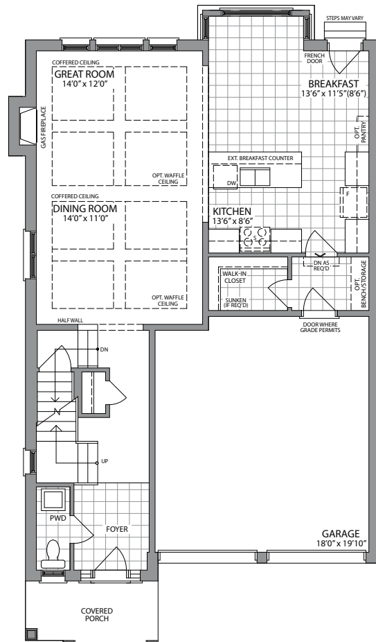
GROUND FLOOR PLAN STYLE 'B'
