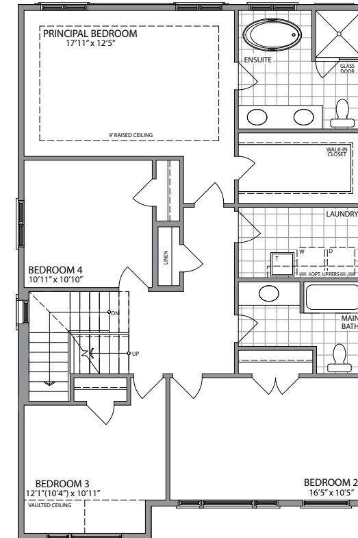
SECOND FLOOR PLAN STYLE 'A'
