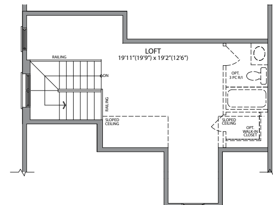
LOFT FLOOR STYLE 'A'
