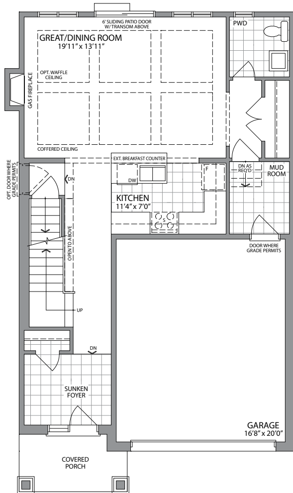
GROUND FLOOR PLAN STYLE 'A'
