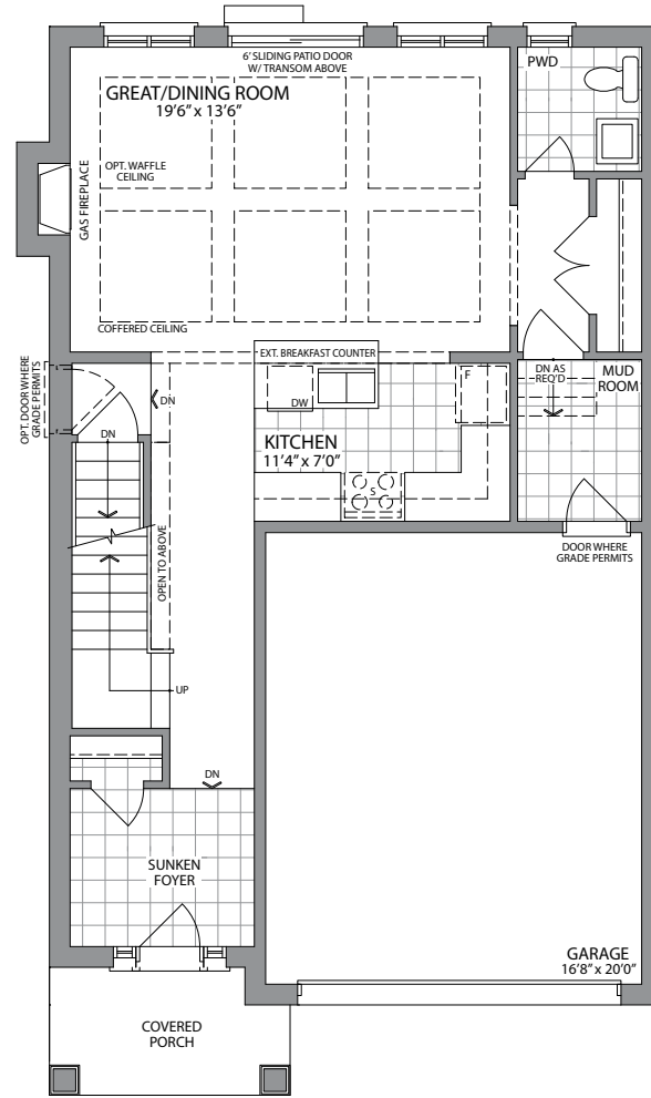
GROUND FLOOR PLAN STYLE 'B'
