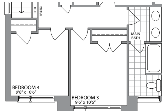
SECOND FLOOR PLAN STYLE 'C'
