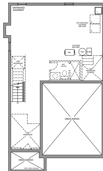
BASEMENT STYLE 'A, B & C'
