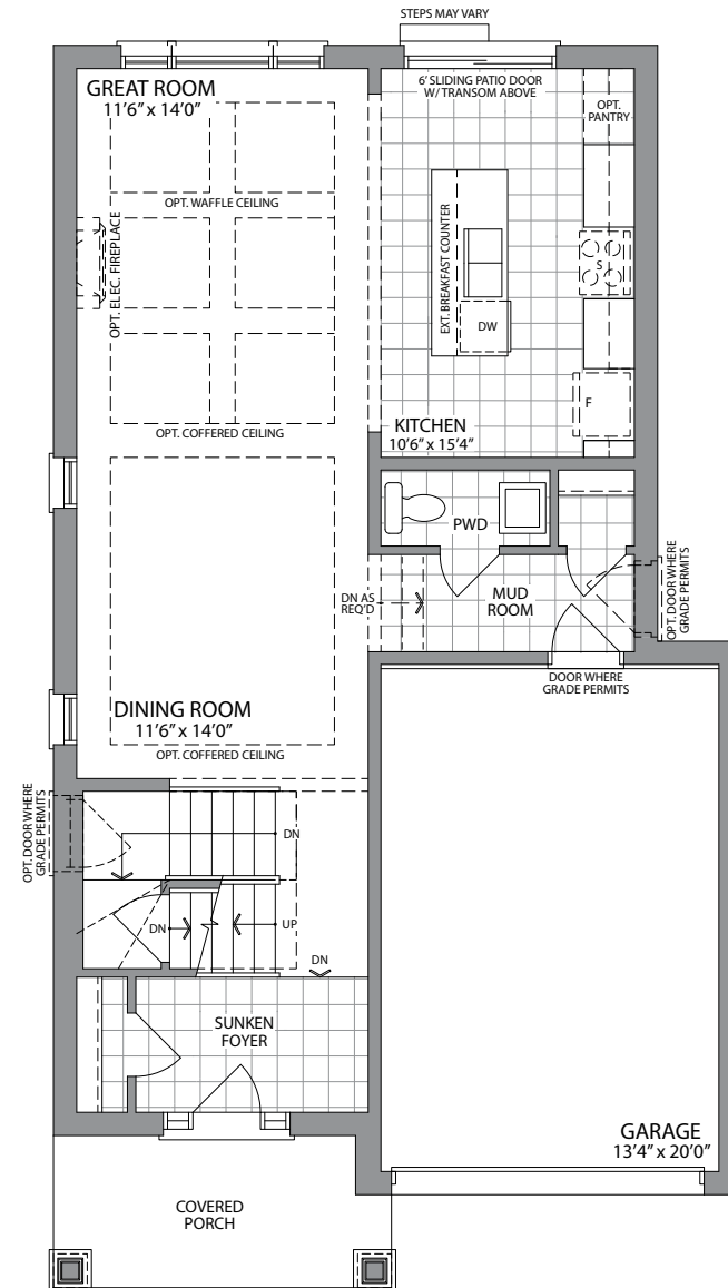
GROUND FLOOR PLAN STYLE 'B'
