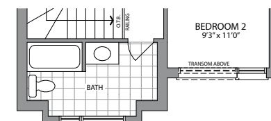
OPT. SECOND FLOOR BATH LAYOUT STYLE 'A'
