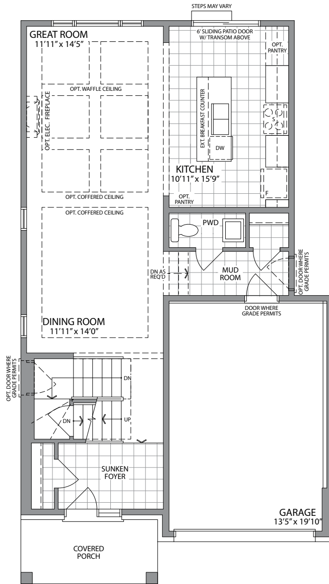
GROUND FLOOR PLAN STYLE 'A'
