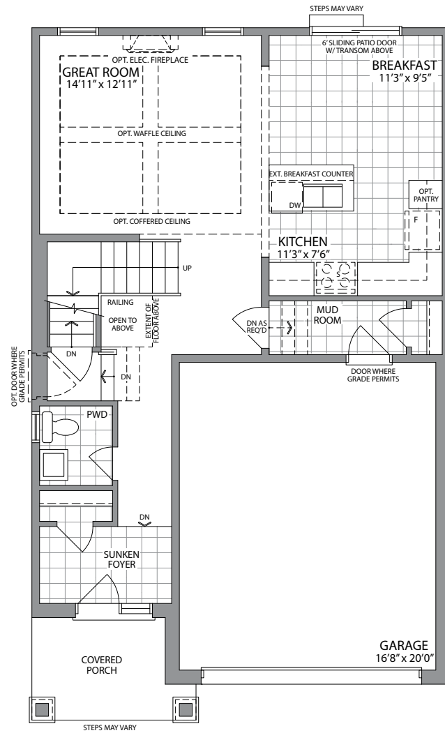
GROUND FLOOR PLAN STYLE 'A'
